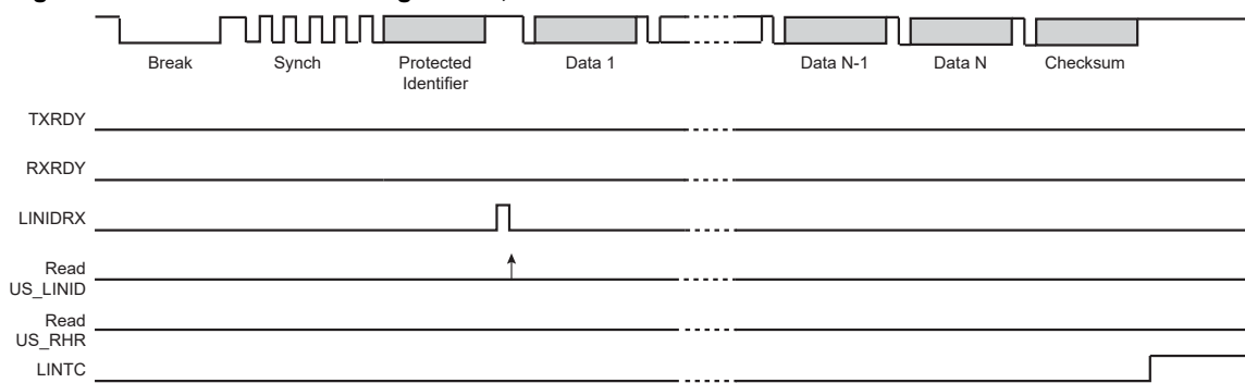
Figure 46-50. Client Node Configuration, NACT = IGNORE
