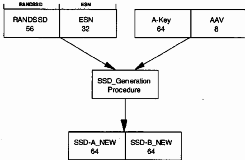
1 Figure 2.3.12-7 Computation of Shared Secret Data
