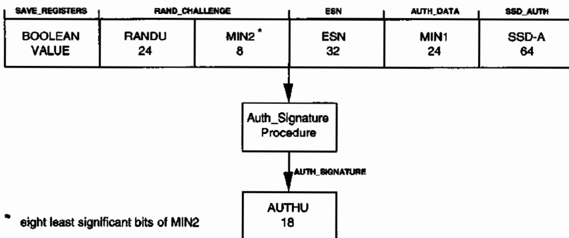
14 Figure 2.3.12-3 Computation of AUTHU
