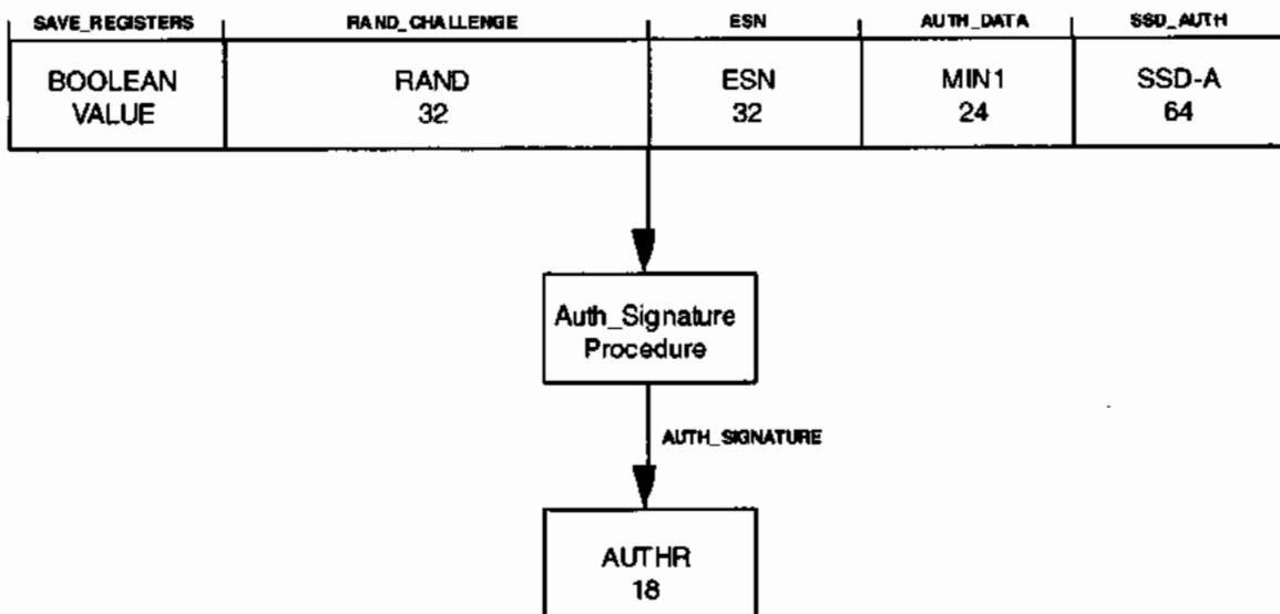
1 Figure 2.3.12-2 Computation of AUTHR for MS Registrations
