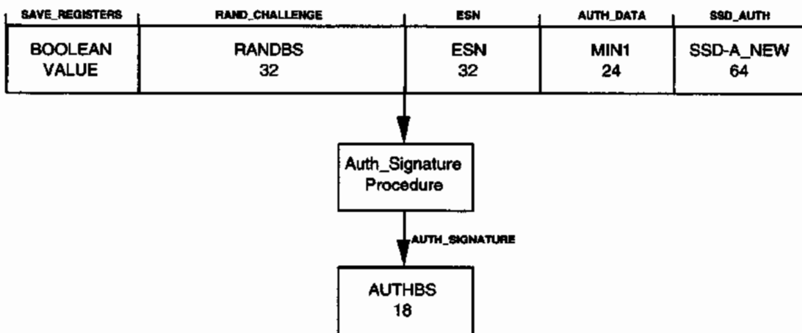
4 Figure 2.3.12-8 Computation of AUTHBS
