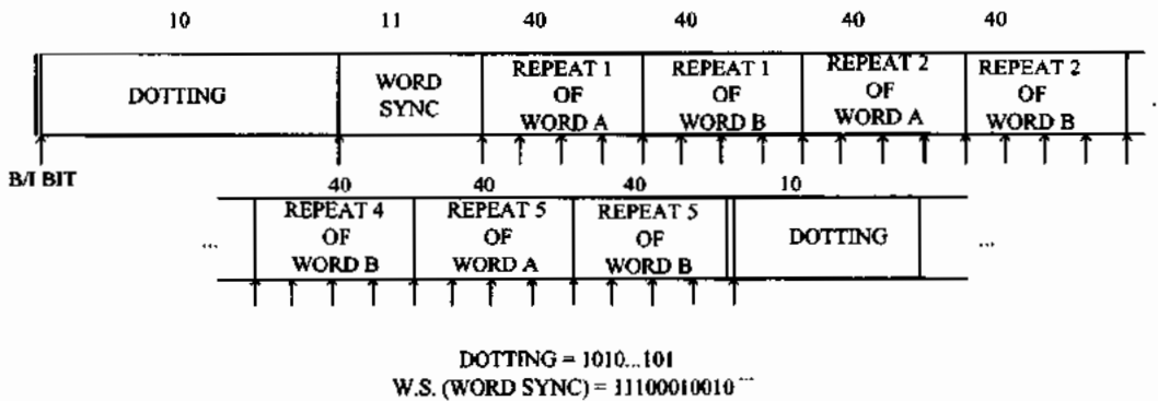
Figure 3.7.1-1 Forward Control Channel Message Stream
