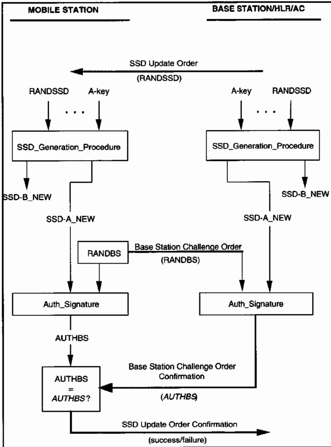
Figure 2.3.12-6 SSD Update Message Flow
